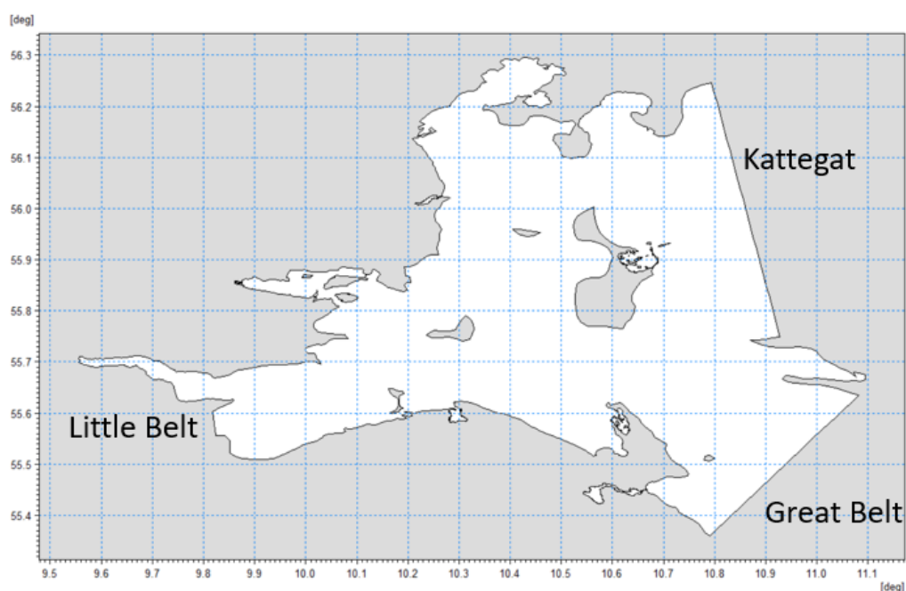
Figure 4.4 Northern Belt Sea model open boundaries
