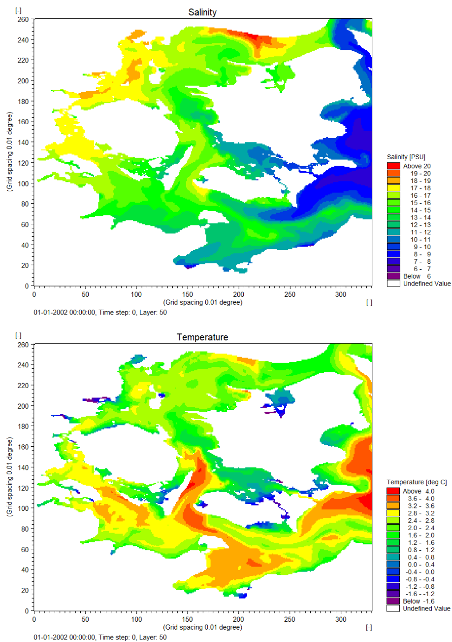
Figure 4.8 Initial surface salinity (top) and temperature (bottom) from the IDF-model used for the Northern Belt Sea model.
