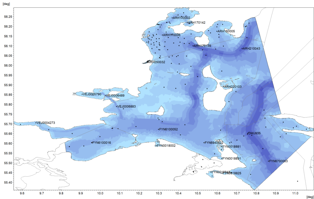
Figure 6.1 Location of monitoring stations in NBS-model domain. Stations used for salinity and temperature validation (ST) are denoted with station name.
