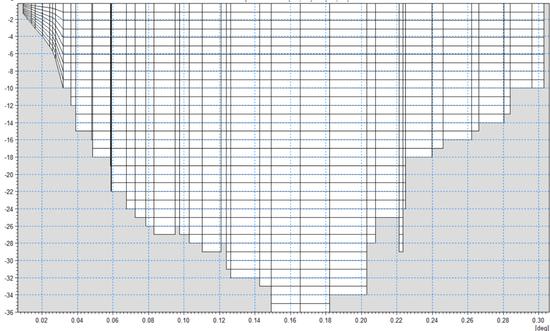
Figure 4.3 Transect within the Northern Belt Sea showing the vertical discretization in the water column: sigma layers down to -10m and 1m z-layers to the seabed. The transect starts at Fynshoved and ends at Røsnæs.
