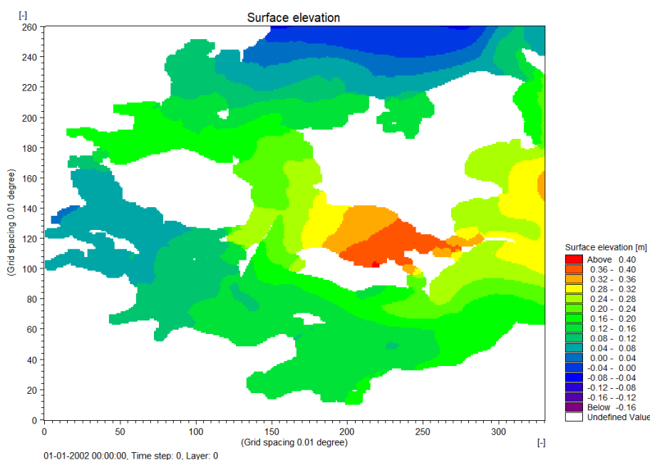
Figure 4.7 Initial 2D map of water level from the IDF-model used as initial fields for the Northern Belt Sea model.
