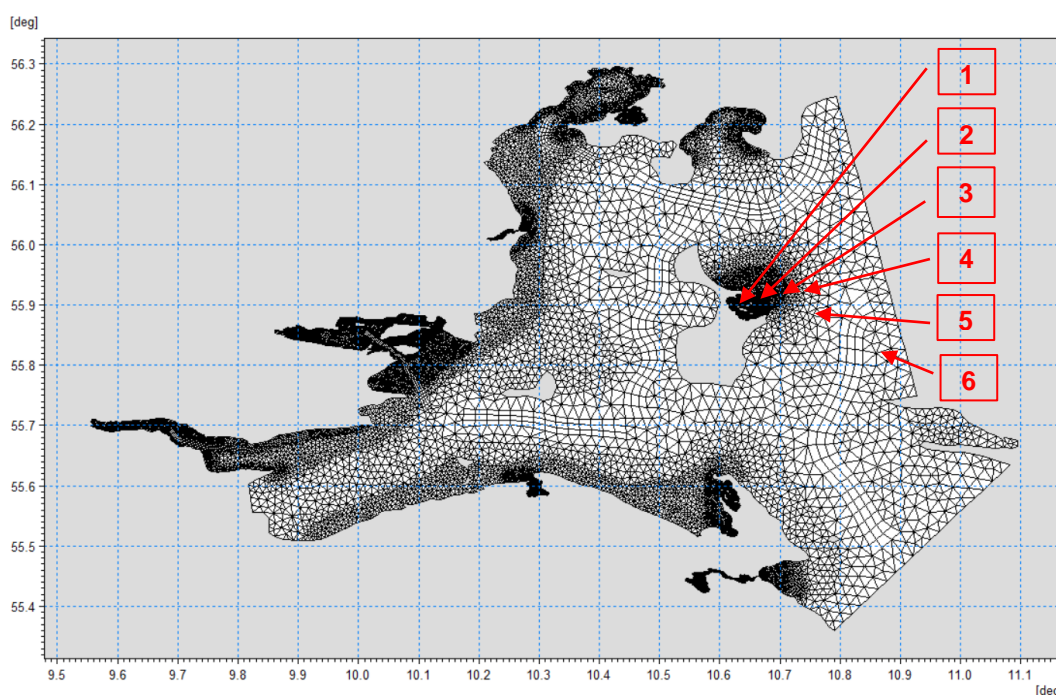
Figure 4.2 NBS-model mesh triangulation including mesh resolution levels from Table 4-1.
