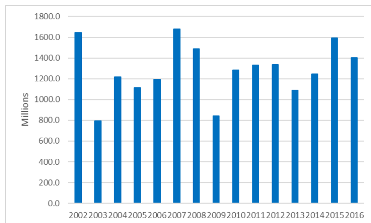
Figure 4.6 Total annual discharge to the NBS-model from the different Danish catchments (million m 3 y -1 ).
