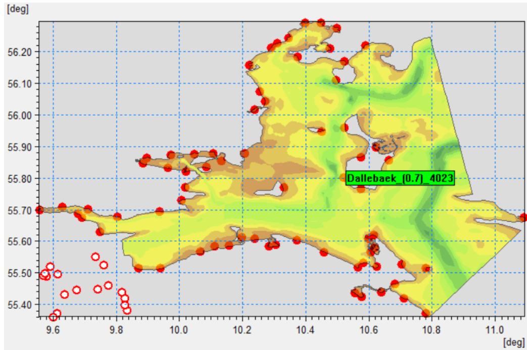
Figure 4.5 Run-off sources included in the Northern Belt Sea model (white dots represents sources located outside the model domain).
