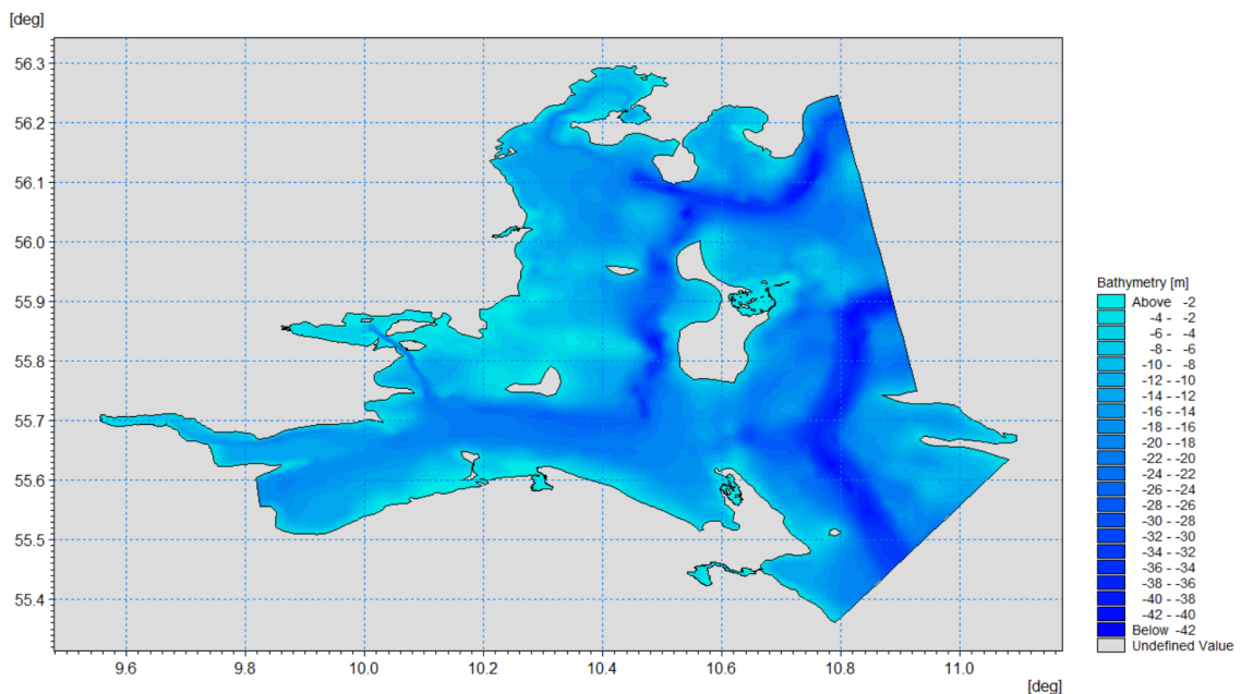
Figure 4.1 Northern Belt Sea model bathymetry. Data originates from Kystdirektorates 50 m bathymetry updated with satellite derived data at shallow waters (DHI 2019b).
