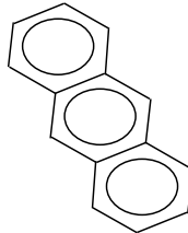
000120-12-7 Anthracene
