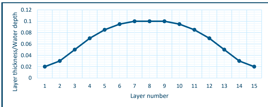
Figure 4.2 Ratio of sigma-layer thickness to water depth, as function of the layer number.
