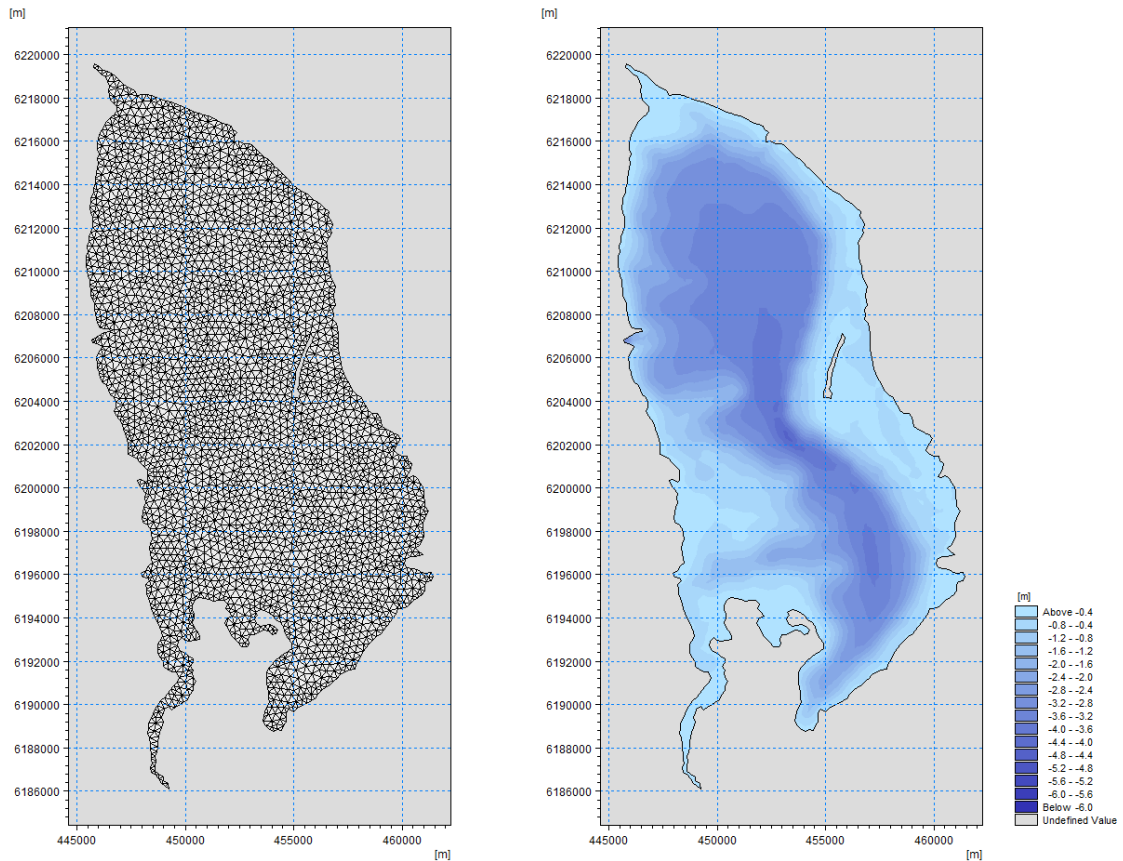
Figure 4.1 (Left) Horizontal mesh and (right) bathymetry of the Ringkøbing Fjord model. Map projection ETRS-1989-UTM-32 and vertical datum DVR90.
