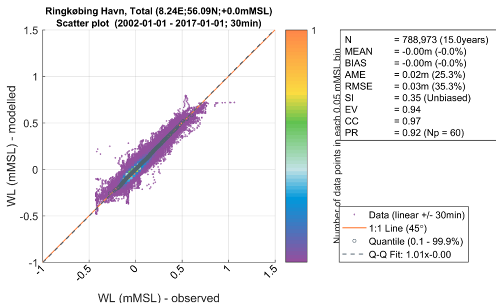
Figure 6.3 Statistical analysis of modelled surface elevation and measured data at Ringkøbing Havn.
