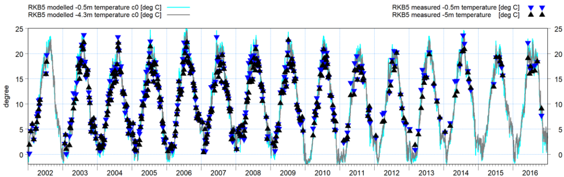
Figure 6.5 Surface and bottom (light blue and grey lines) model temperature at station RKB5 compared to measured surface and bottom (blue and black triangles) values.
