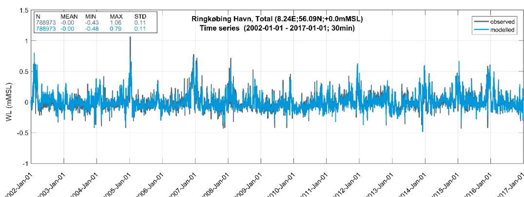
Figure 6.2 Modelled surface elevation (light blue line) compared to measured data (dark blue line) at Ringkøbing Havn.
