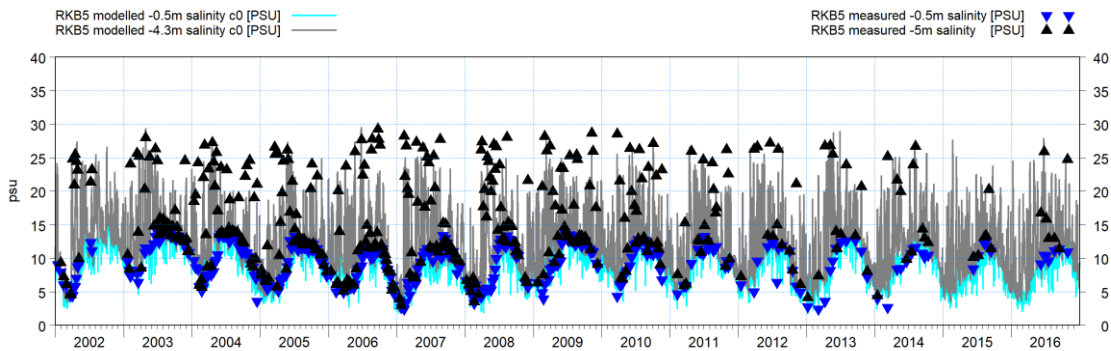
Figure 6.4 Surface and bottom (light blue and grey lines) model salinity at station RKB5 compared to measured surface and bottom (blue and black triangles) values.
