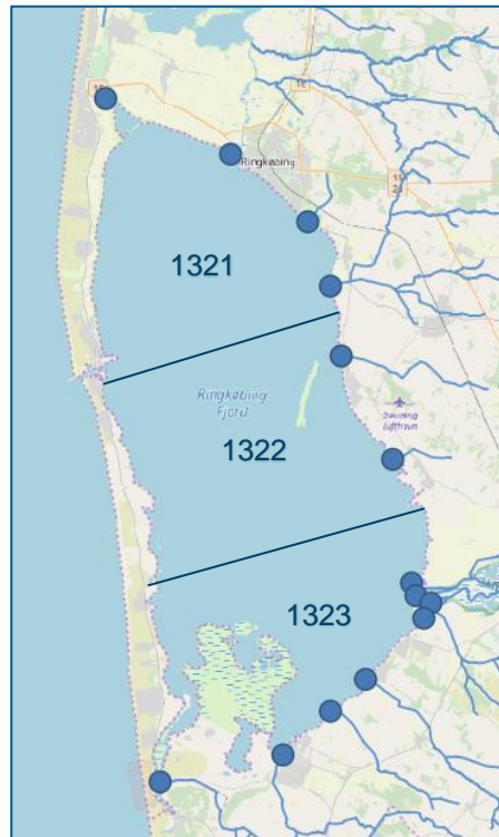
Figure 4.4 Location of freshwater sources and subdivision of Ringkøbing Fjord into three areas (1321, 1322, 1323), for which total daily discharge time series were distributed to the sources.
