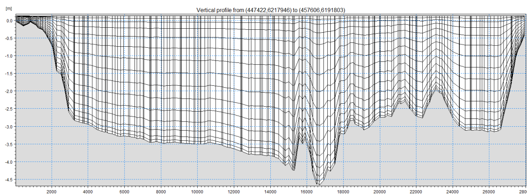
Figure 4.3 Vertical model mesh of the Ringkøbing Fjord model in transect from north-west to south-east, with 15 sigma-layers refined towards the surface and fjord bed.
