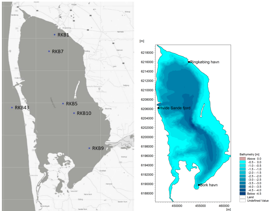
Figure 6.1 Location of the validation stations for salinity and temperature (left) and water level (right) used in the model performance.
