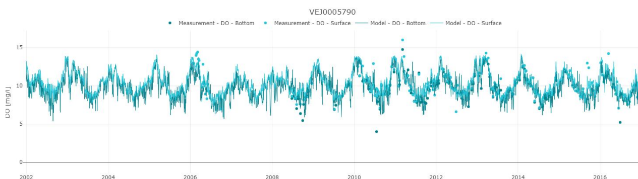
Figure 5-6 Comparison of measured and modelled concentrations of dissolved oxygen (mg/l) at station VEJ0005790 in the surface and bottom (3 m) waters. Dots represent measurements, and the solid line shows modelled data for the entire period.
