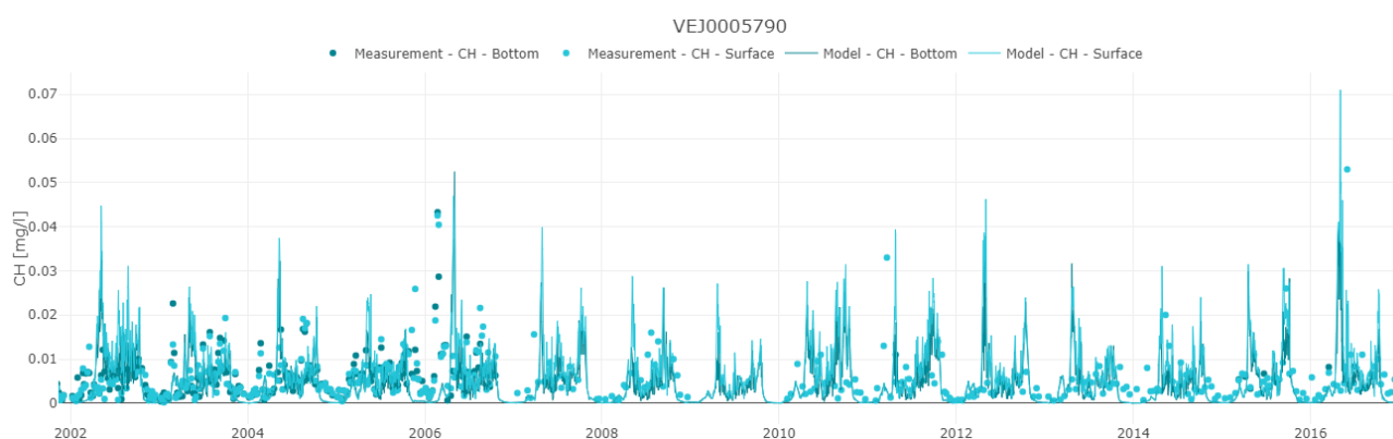
Figure 5-7 Comparison of measured and modelled concentrations of chlorophyll-a (mg/l) at station VEJ0005790 in surface and bottom (3 m) waters. Dots represent measurements, and solid lines show modelled data for the entire period.
