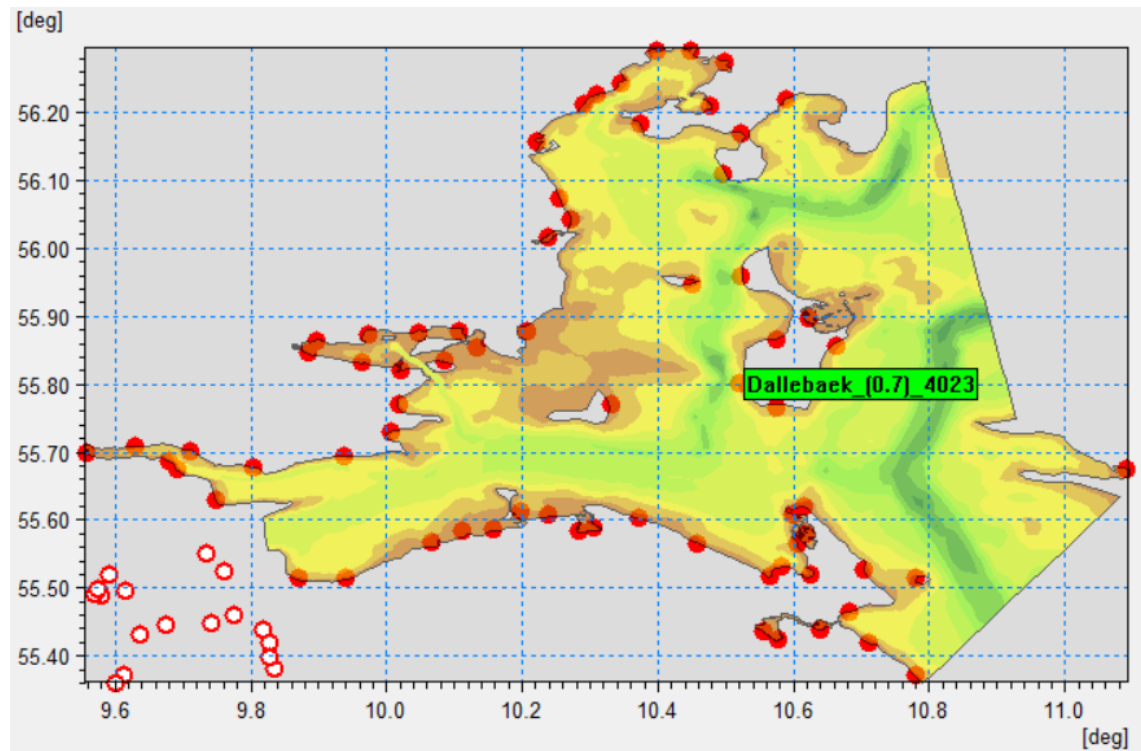
Figure 4-3 Run-off sources included in the Northern Belt Sea model (white dots represent sources not included in model calculations).
