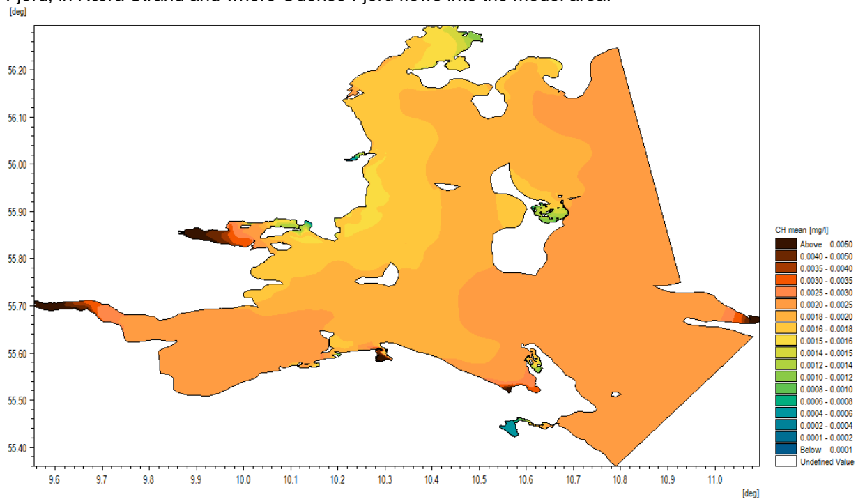
Figure 5-2 Modelled annual average surface water concentrations of chlorophyll-a (mg/l) for 2016.
