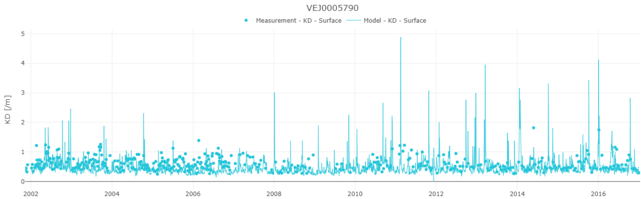
Figure 5-8 Comparison of measured and modelled light attenuation coefficient ( K_d ) at station VEJ0005790 in the surface waters. Dots represent measurements, and the solid line shows modelled data for the entire period.
