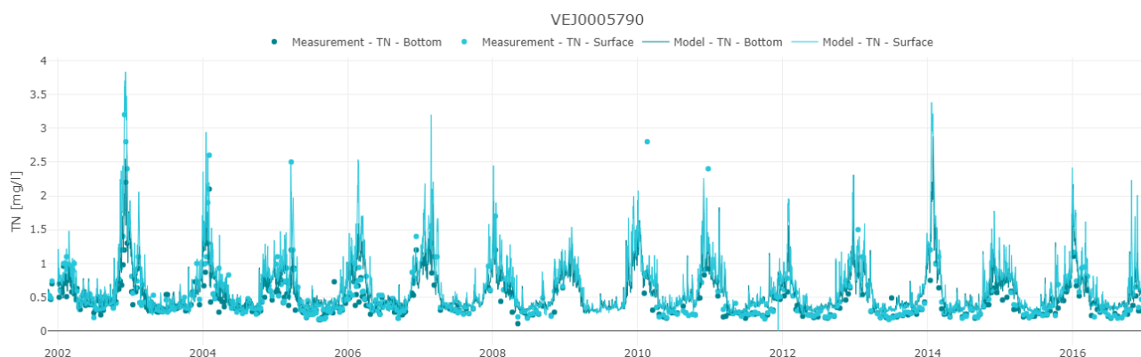
Figure 5-11 Comparison of measured and modelled concentrations of total nitrogen (TN) at station VEJ0005790 in surface and bottom (3 m) waters. Scatter data represent measurements, and solid lines show modelled data for the entire period.
