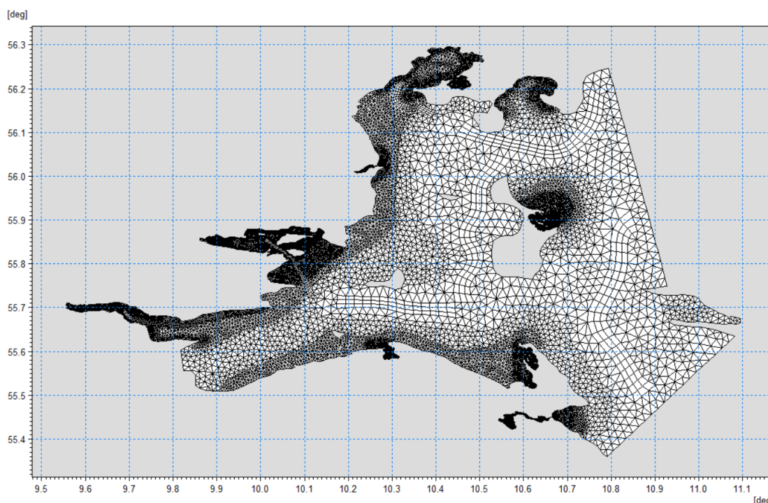
Figure 4-2 Resolution of the horizontal model mesh of the NBH model.
