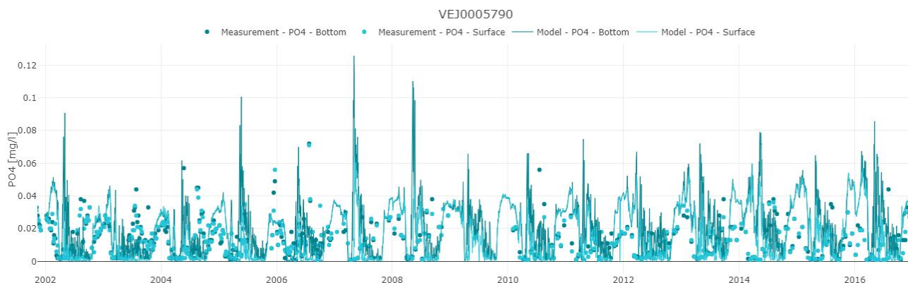
Figure 5-10 Measured and modelled concentrations of dissolved inorganic phosphorus (DIP) at station VEJ0005790 in the surface and bottom (3 m) waters. Dots represent measurements, and solid lines show modelled data for the entire period.
