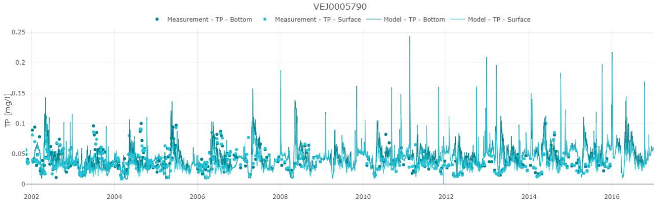
Figure 5-12 Comparison of measured and modelled concentrations of total P (TP) at station VEJ0005790 in surface and bottom (3 m) waters. Scatter data represent measurements, and solid lines show modelled data for the entire period.
