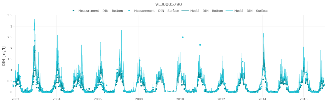
Figure 5-9 Measured and modelled concentrations of dissolved inorganic nitrogen (DIN) at station VEJ0005790 in the surface and bottom (3 m) waters. Dots represent measurements, and solid lines show modelled data for the entire period.
