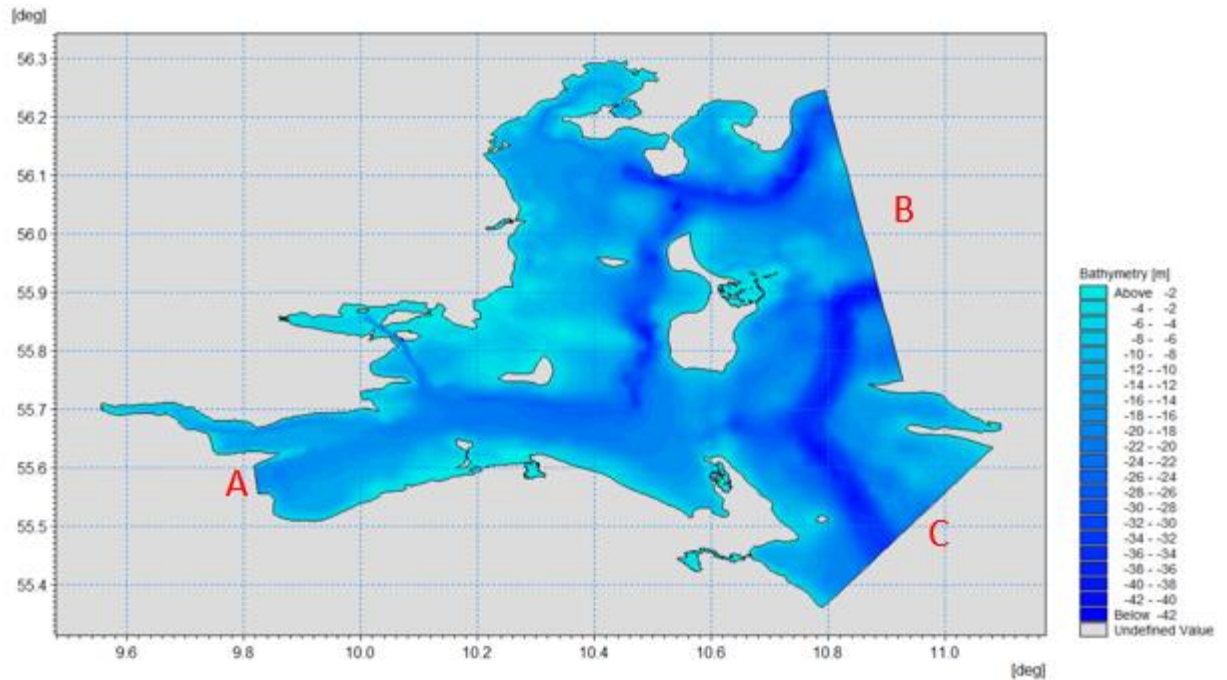
Figure 4-1 Top: Northern Belt Sea model bathymetry. Data originates from Kystdirektoratets 50 m bathymetry updated with satellite-derived data at shallow waters (DHI 2019e). The model includes three open boundaries connecting the model area to surrounding water bodies. A) Little Belt boundary, B) Kattegat boundary, C) Great Belt boundary.
