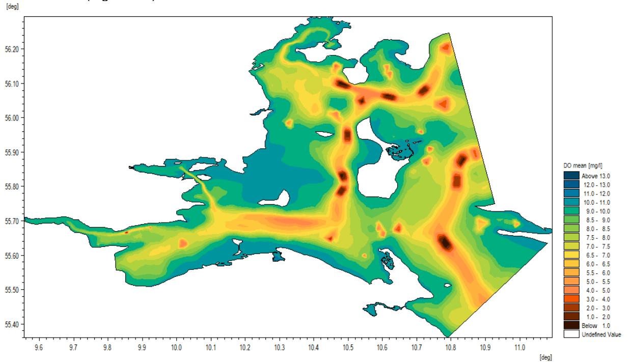
Figure 5-1 Modelled annual average bottom water concentrations of dissolved oxygen (mg/l) for 2016.
