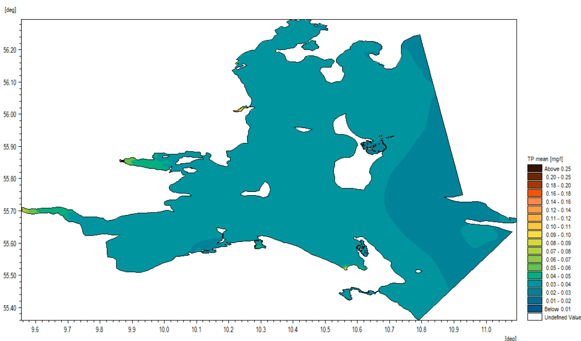
Figure 5-4 Modelled yearly average surface water concentrations of total phosphorus (mg/l) for 2016.
