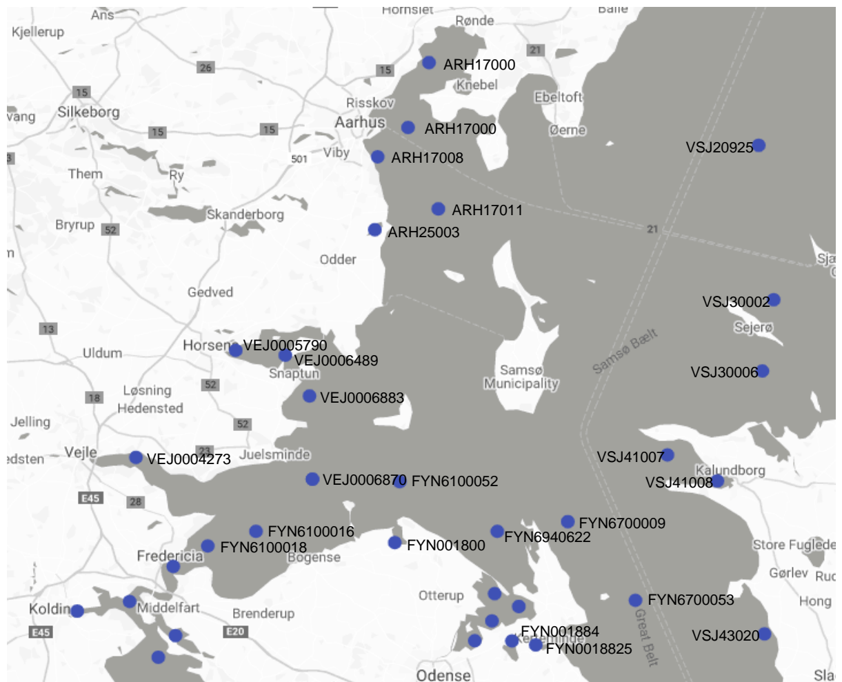
Figure 5-5 Stations within the NBH-model domain (only stations with ID).
