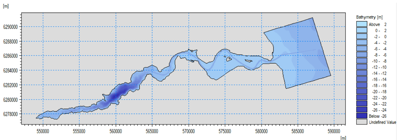
Figure 4-1 Model bathymetry of the Mariager Fjord model. The model has one open boundary with three sections towards Kattegat. Map projection ETRS-1989-UTM-32 and vertical datum DVR90.
