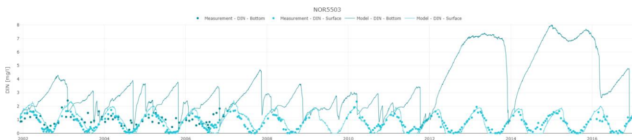
Figure 5-9 Measured and modelled concentrations of dissolved inorganic nitrogen (DIN, mg/l) at station NOR5503 in the surface and bottom (15 m) waters. Dots represent measurements, and solid lines show modelled data for the entire period.
