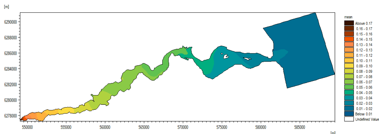
Figure 5-4 Modelled yearly average surface water concentrations of total phosphorus (TP, mg/l) in 2016.
