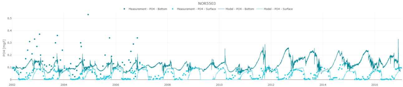
Figure 5-10 Measured and modelled concentrations of dissolved inorganic phosphorus (DIP, mg/l) at station NOR5503 in the surface and bottom (15 m) waters. Dots represent measurements, and solid lines show modelled data for the entire period.
