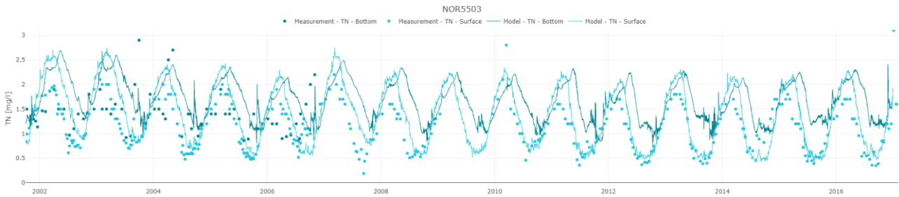
Figure 5-11 Comparison of measured and modelled concentrations of total nitrogen (TN, mg/l) at station NOR5503 in surface and bottom (15 m) waters. Scatter data represent measurements, and solid lines show modelled data for the entire period.
