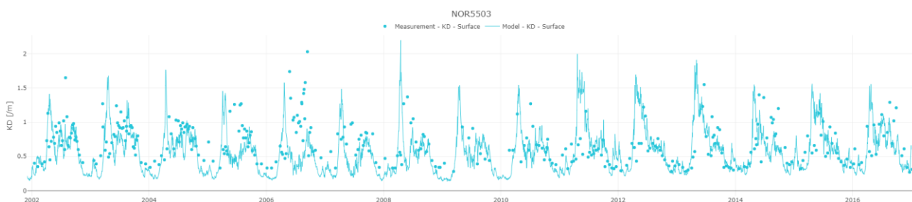
Figure 5-8 Comparison of measured and modelled light attenuation coefficient ( K_d , m^{-1} ) at station NOR5503 in the surface waters. Dots represent measurements, and the solid line shows modelled data for the entire period.
