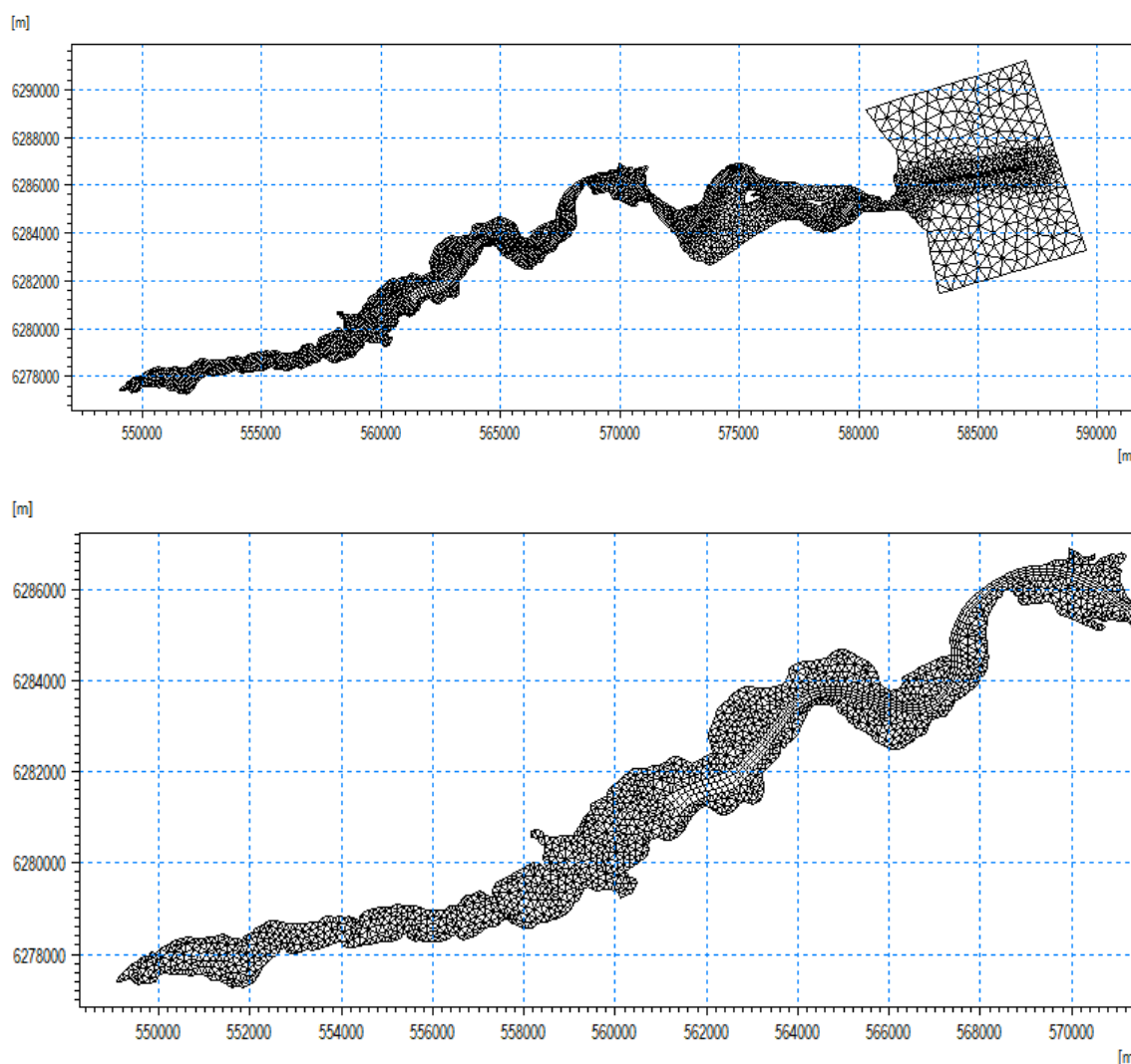
Figure 4-2 Resolution of the horizontal model mesh of the Mariager Fjord model. Upper showing full model. Lower showing inner fjord resolution.
