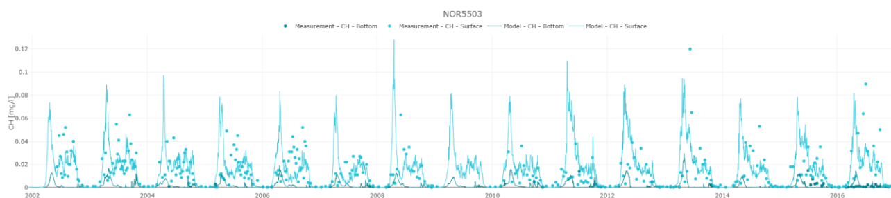
Figure 5-7 Comparison of measured and modelled concentrations of chlorophyll-a (CH, mg/l) at station NOR5503 in surface and bottom (15 m) waters. Dots represent measurements, and solid lines show modelled data for the entire period.
