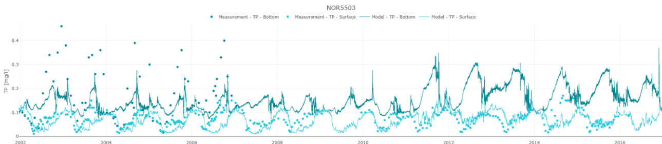
Figure 5-12 Comparison of measured and modelled concentrations of total P (TP, mg/l) at station NOR5503 in surface and bottom (15 m) waters. Scatter data represent measurements, and solid lines show modelled data for the entire period.
