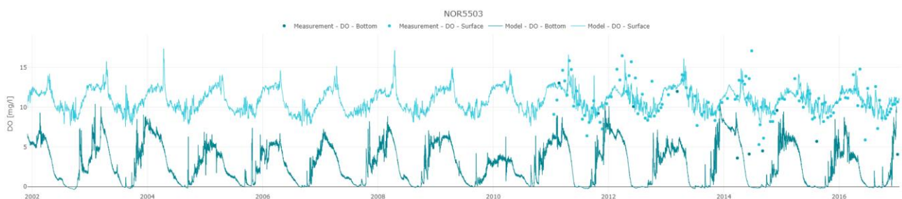
Figure 5-6 Comparison of measured and modelled concentrations of dissolved oxygen (DO, mg/l) at station NOR5503 in the surface and bottom (15 m) waters. Dots represent measurements, and the solid line shows modelled data for the entire period.
