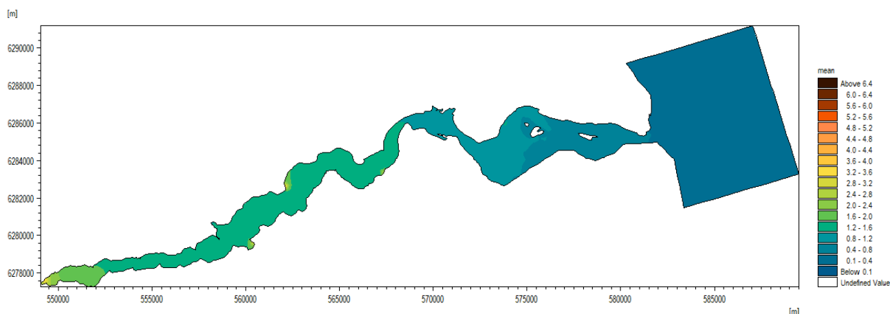
Figure 5-3 Modelled yearly average surface water concentrations of total nitrogen (TN, mg/l) in 2016.
