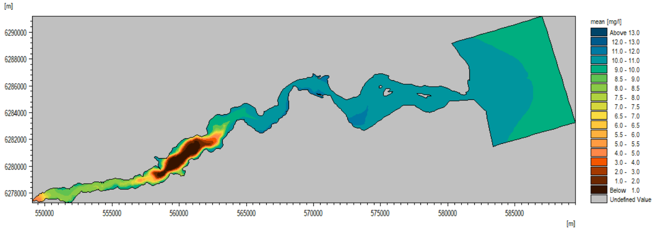
Figure 5-1 Modelled yearly average bottom water concentrations of dissolved oxygen (DO, mg/l) for 2016.
