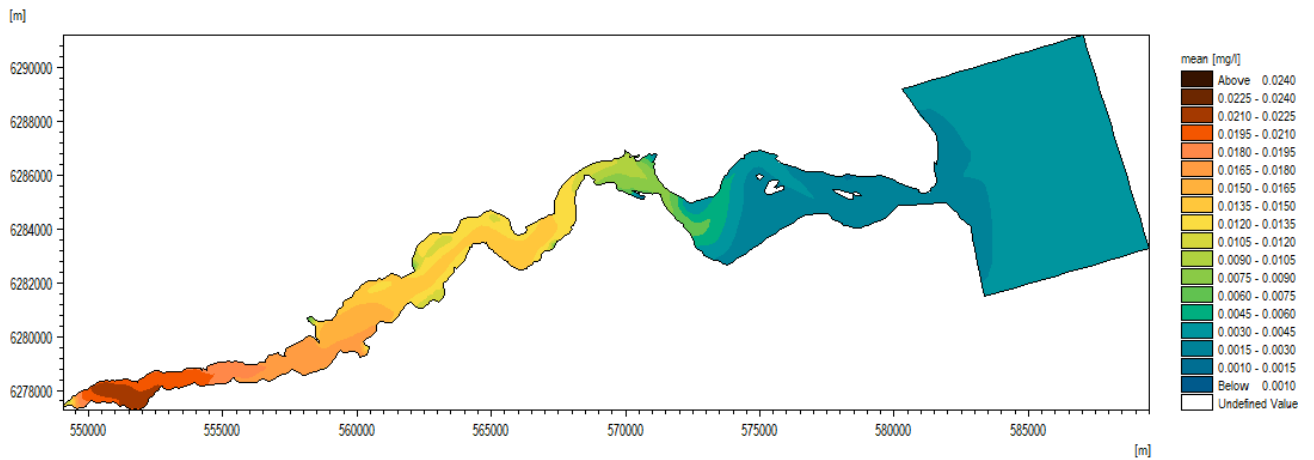
Figure 5-2 Modelled yearly average surface water concentrations of chlorophyll-a (CH, mg/l) for 2016.
