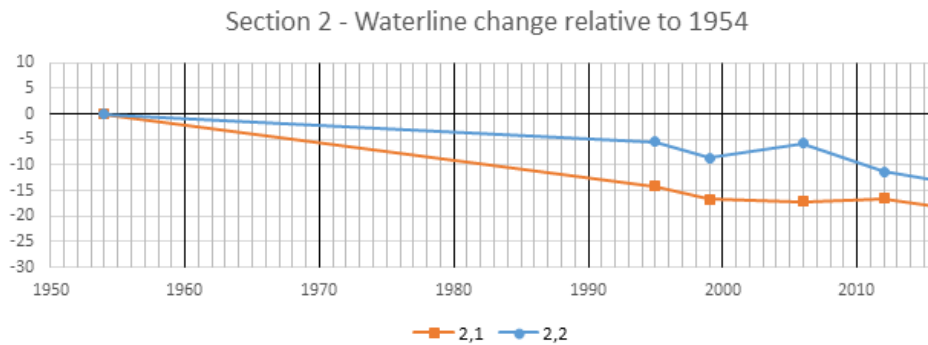
Figure 4.3: Showing the measured shoreline position for the included years, relative to the 1954 position.
