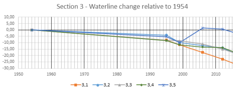
Figure 4.4: Showing the measured shoreline position for the included years, relative to the 1954 position.
