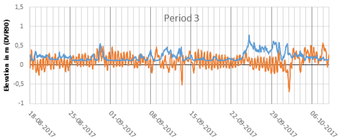
Figure 5.5: Modelled wave height and water level from the DMI dataset for period 3. Note that SWH is short for "significant wave height".
