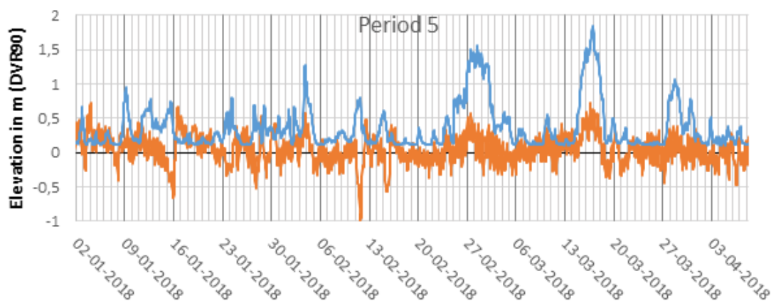
Figure 5.8: Modelled wave height and water level from the DMI dataset for period 5. Note that SWH is short for "significant wave height".
