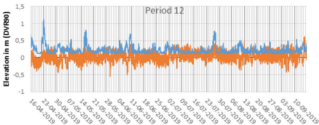
Figure 5.15: Modelled wave height and water level from the DMI dataset for period 12. Note that SWH is short for "significant wave height".
