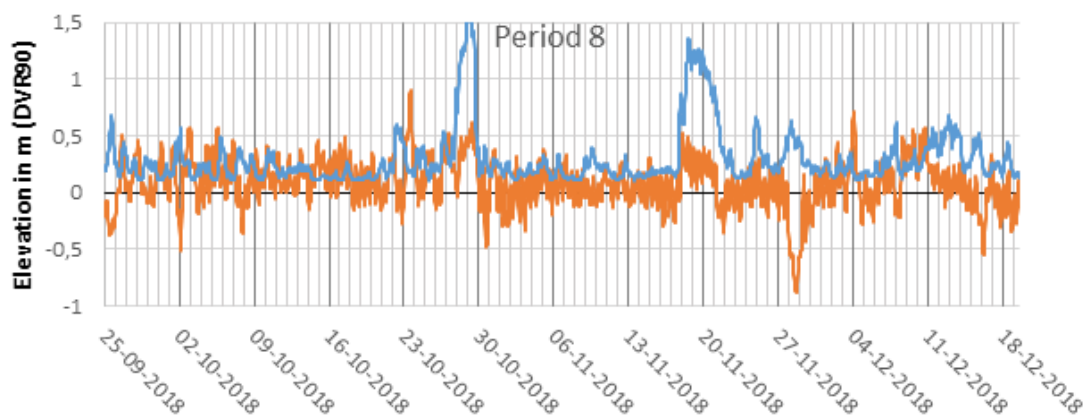
Figure 511: Modelled wave height and water level from the DMI dataset for period 8. Note that SWH is short for "significant wave height".
