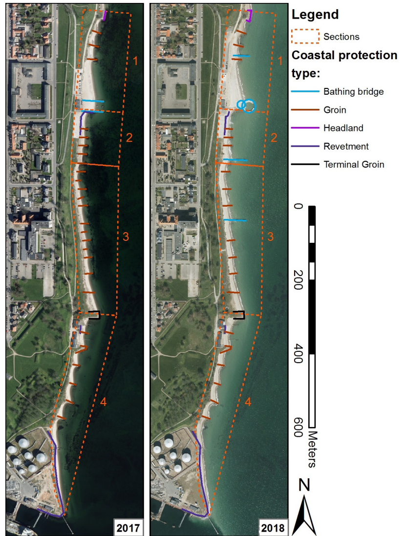
Figure 5.2: Passive hard coastal protection measure before and after the beach nourishment.
