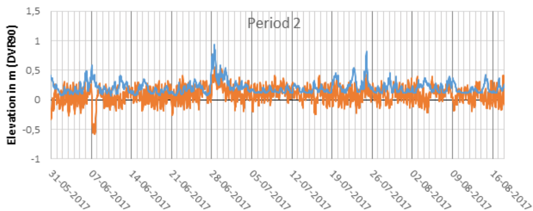
Figure 5.4: Modelled wave height and water level from the DMI dataset for period 2. Note that SWH is short for "significant wave height".
