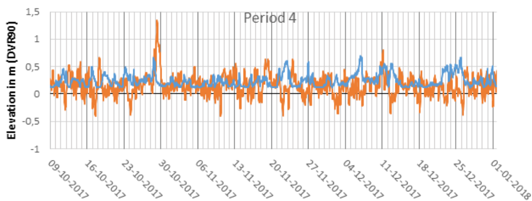
Figure 5.7: Modelled wave height and water level from the DMI dataset for period 4. Note that SWH is short for "significant wave height".
