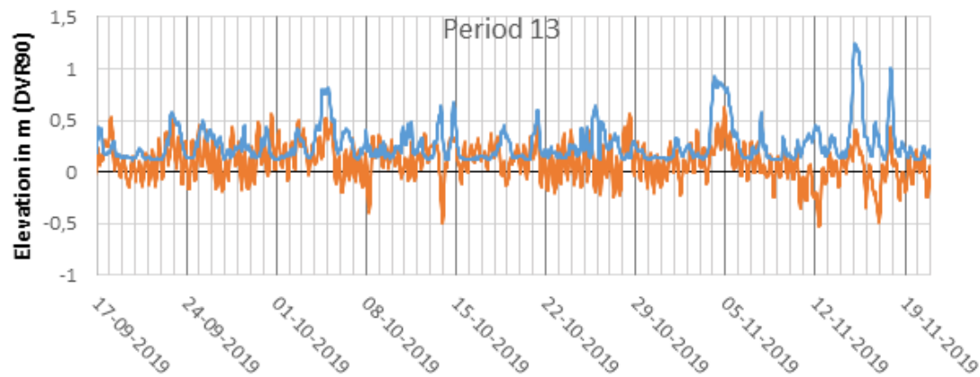
Figure 5.16: Modelled wave height and water level from the DMI dataset for period 13. Note that SWH is short for "significant wave height".
