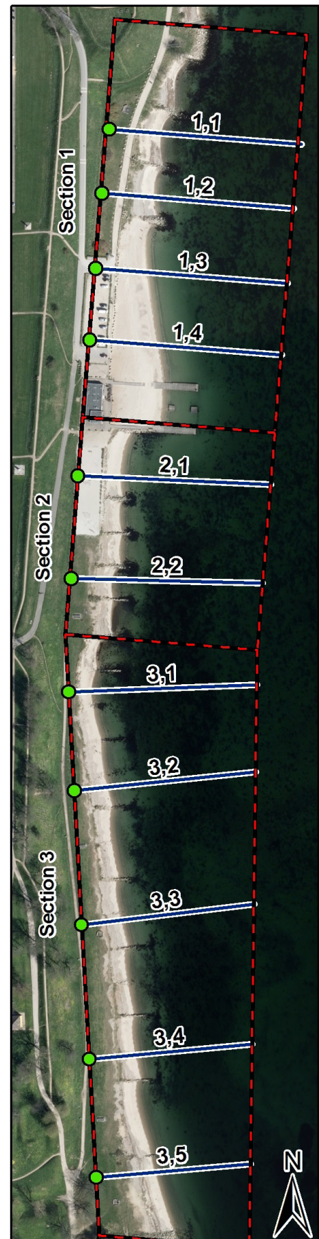
Figure 3.3: Profile lines drawn for estimation of shoreline retreat.
