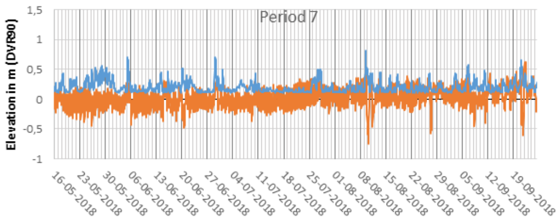
Figure 510: Modelled wave height and water level from the DMI dataset for period 7. Note that SWH is short for "significant wave height".
