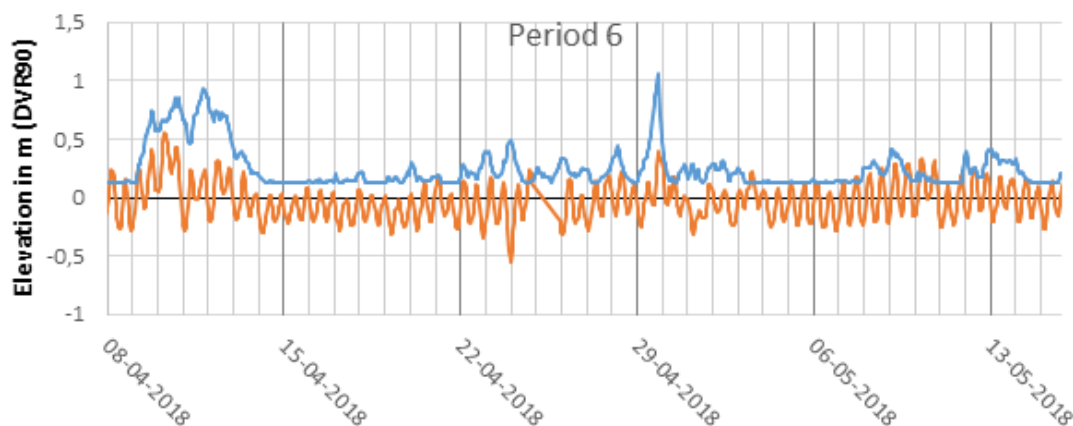
Figure 5.9: Modelled wave height and water level from the DMI dataset for period 6. Note that SWH is short for "significant wave height".
