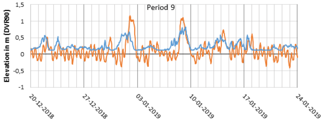
Figure 5.12: Modelled wave height and water level from the DMI dataset for period 9. Note that SWH is short for "significant wave height".
