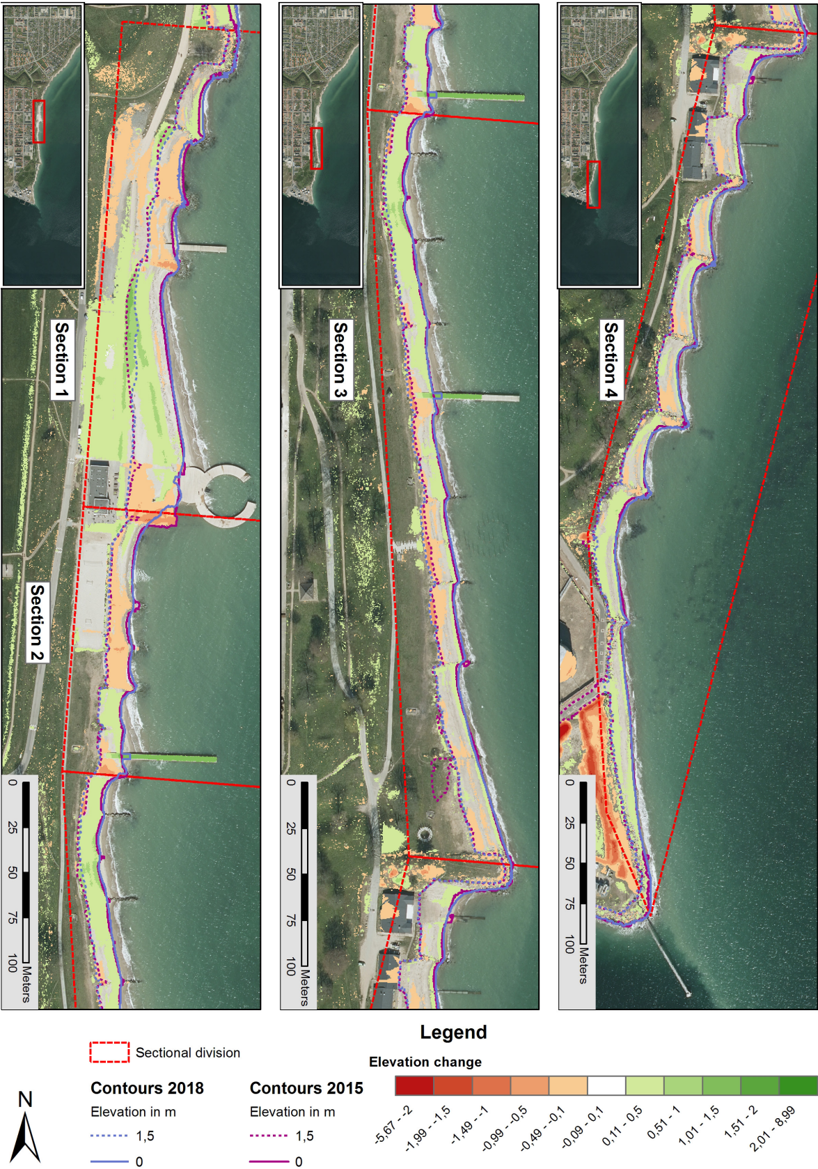
Figure 518: Difference mapping between the two national terrain elevation models. The beach volumes are quantified within the total extent of the 1,5m contours and 0m contours in table 3.5.
