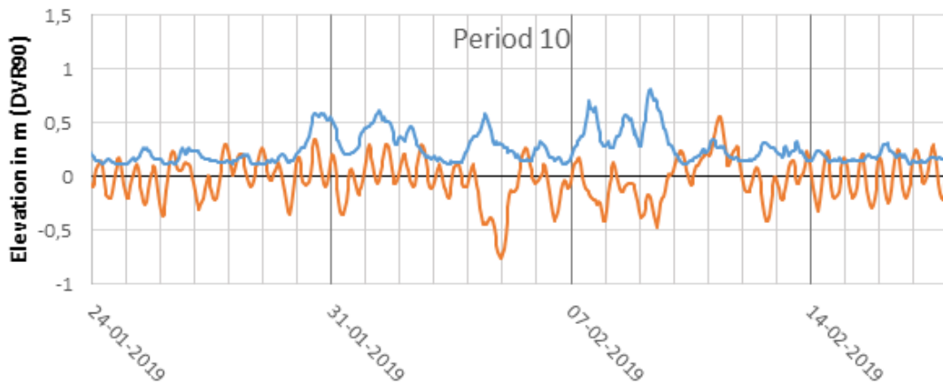
Figure 5.13: Modelled wave height and water level from the DMI dataset for period 10. Note that SWH is short for "significant wave height".
