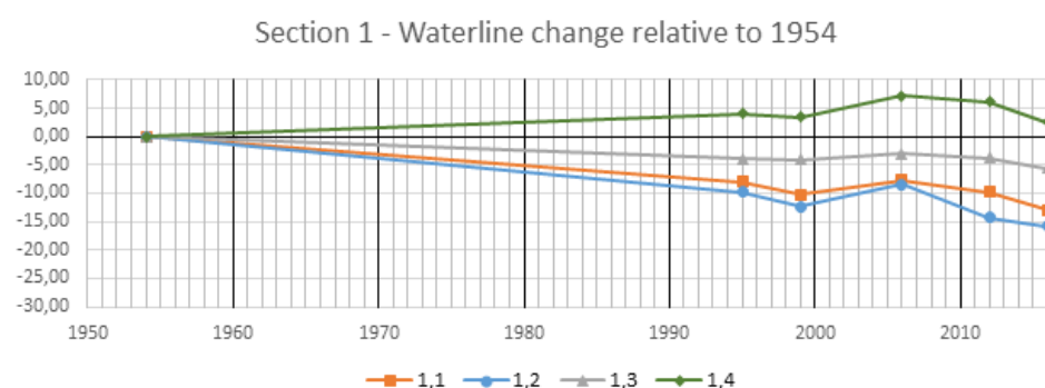
Figure 4.2: Showing the measured shoreline position for the included years, relative to the 1954 position.
