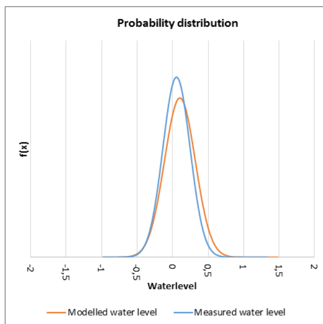
Fig. 2.2: Probability density distribution for modelled and measured water levels.
