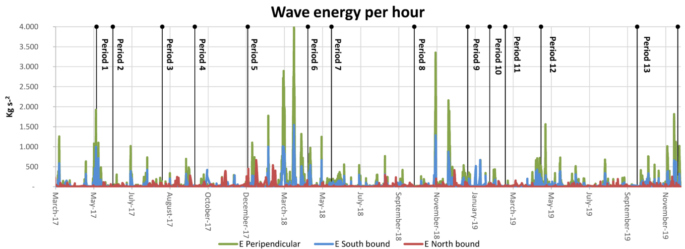
Figure 5.1: The wave energy alongshore (north/south) and perpendicularly is calculated every hour from the method described in Chapter 3. Division into periods is represented as black vertical lines with the respective date attached.
