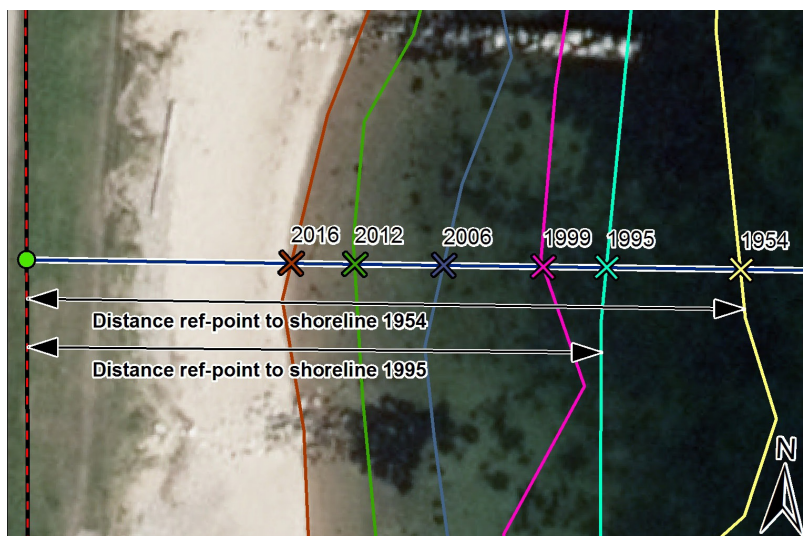
Figure 3.4: The intersections marked with crosses are created as described in the text. Here the shoreline retreat would be found as: Retreat from 1954 to 1995 = Distance 1954 - Distance 1995.
