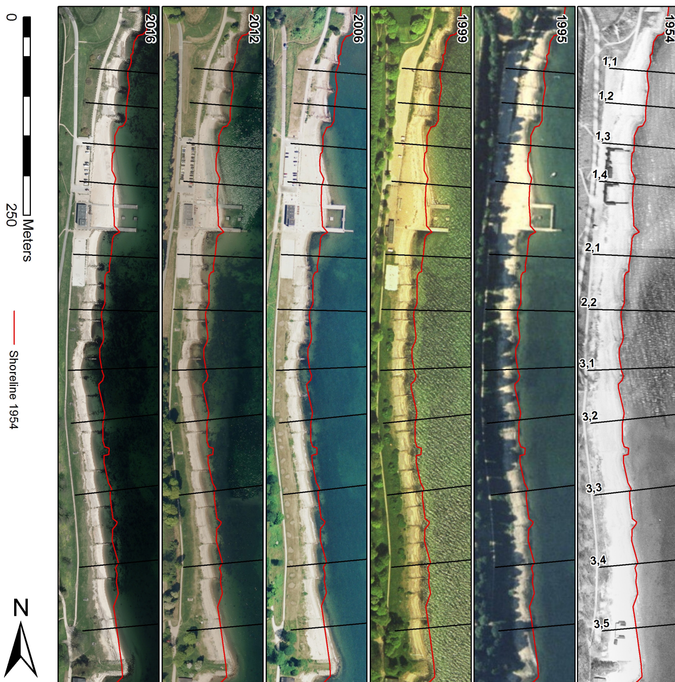
Figure 41: Time stack of Orthophotos at Østerstrand, Fredericia. The Shoreline polyline in red are drawn by hand as the approximate boundary between sand and water on the 1954 imagery.
