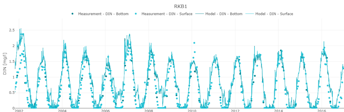
Figure 5-9 Measured and modelled concentrations of dissolved inorganic nitrogen (DIN, mg/l) at station RKB1 in the surface and bottom (3 m) waters. Dots represent measurements, and solid lines show modelled data for the entire period.
