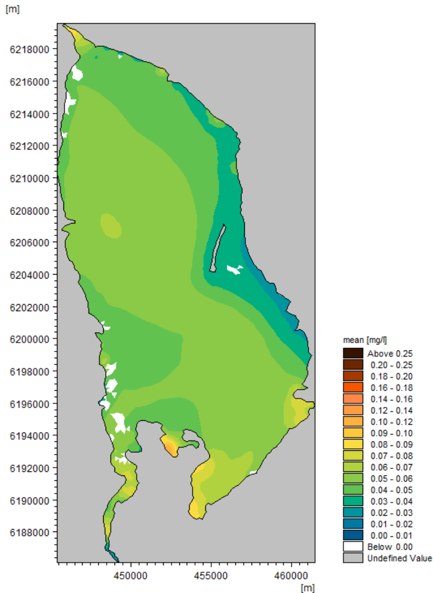
Figure 5-4 Modelled yearly average surface water concentrations of total phosphorus (TP, mg/l) for 2016.
