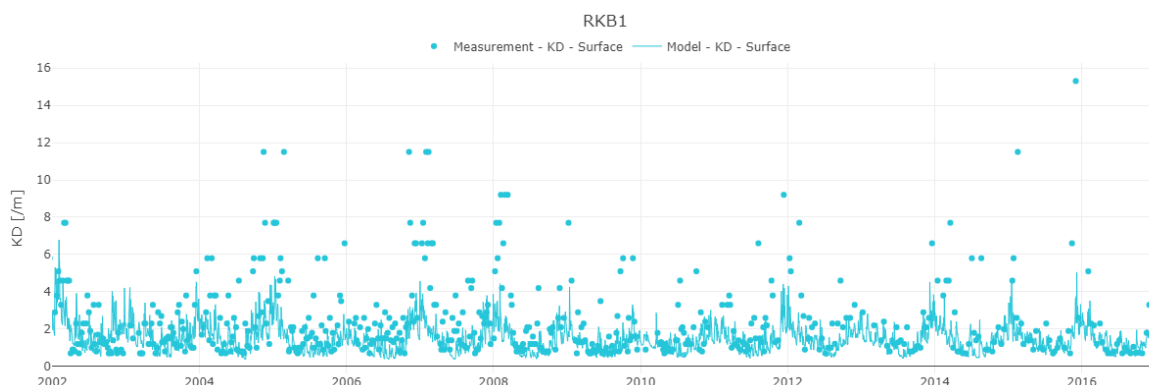
Figure 5-8 Comparison of measured and modelled light attenuation coefficient ( K_d , m^{-1} ) at station RKB1 in the surface waters. Dots represent measurements, and the solid line shows modelled data for the entire period.
