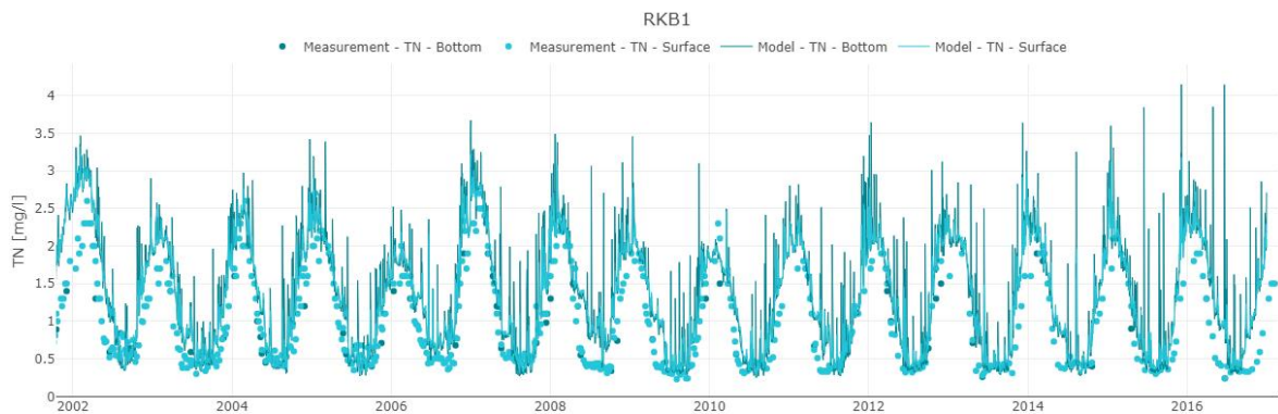
Figure 5-11 Comparison of measured and modelled concentrations of total nitrogen (TN, mg/l) at station RKB1 in surface and bottom (3 m) waters. Scatter data represent measurements, and solid lines show modelled data for the entire period.
