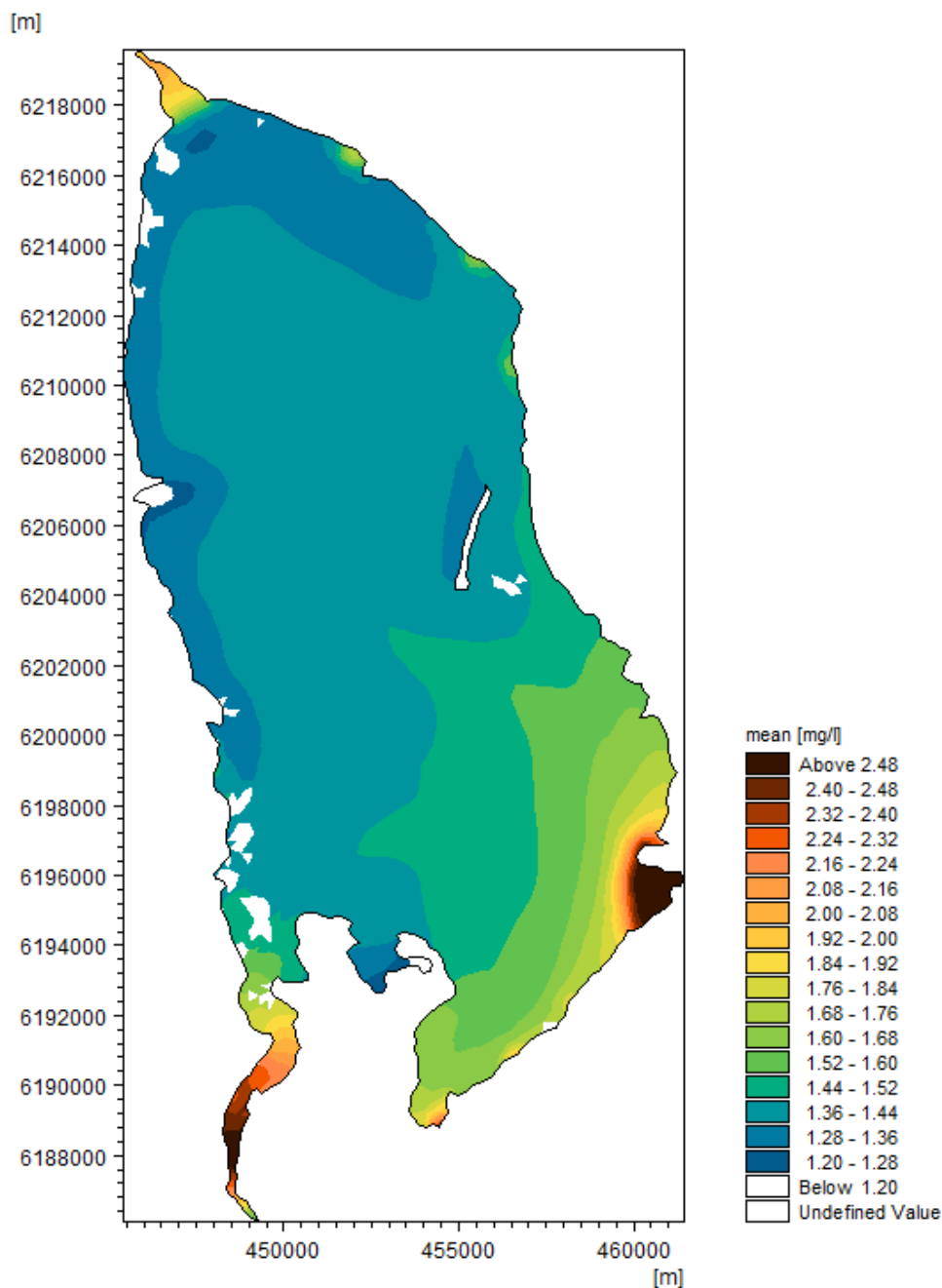
Figure 5-3 Modelled yearly average surface water concentrations of total nitrogen (TN, mg/l) for 2016.
