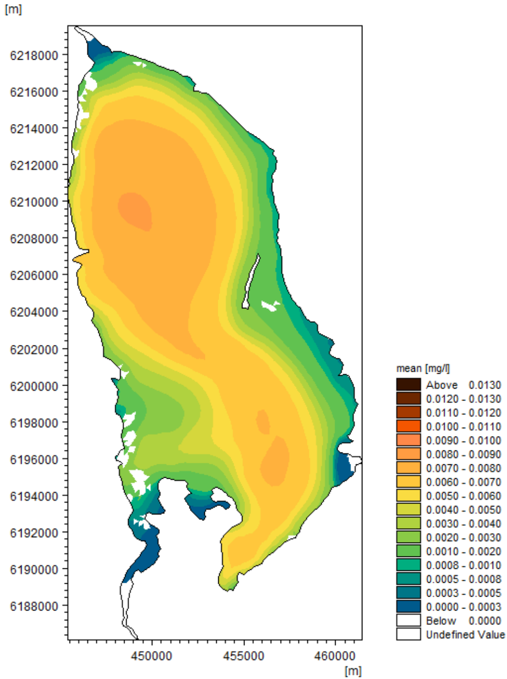
Figure 5-2 Modelled yearly average surface water concentrations of chlorophyll-a (CH, mg/l) for 2016.
