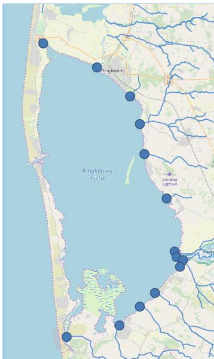
Figure 4-3 Location of sources in the Ringkøbing Fjord model. The sources positions represent the main rivers, but loadings are scaled to include all local run-off and point sources from land to the fjord.
