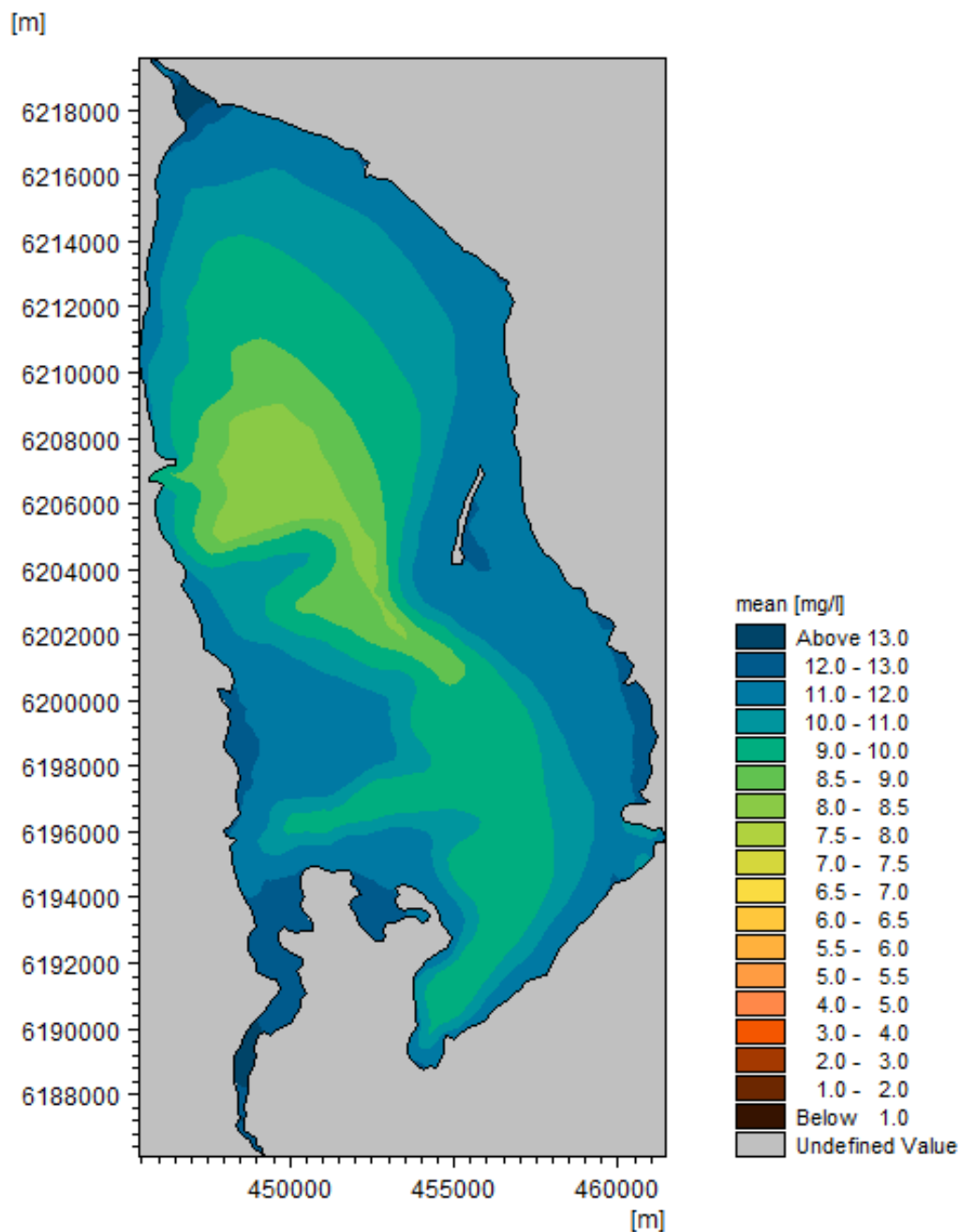
Figure 5-1 Modelled yearly average bottom water concentrations of dissolved oxygen (DO, mg/l) for 2016.
