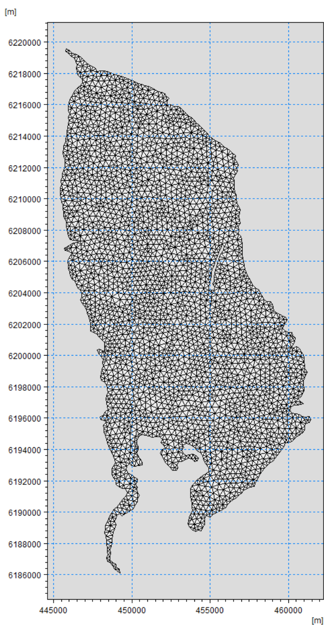
Figure 4-2 Resolution of the horizontal model mesh of the Ringkøbing Fjord model.
