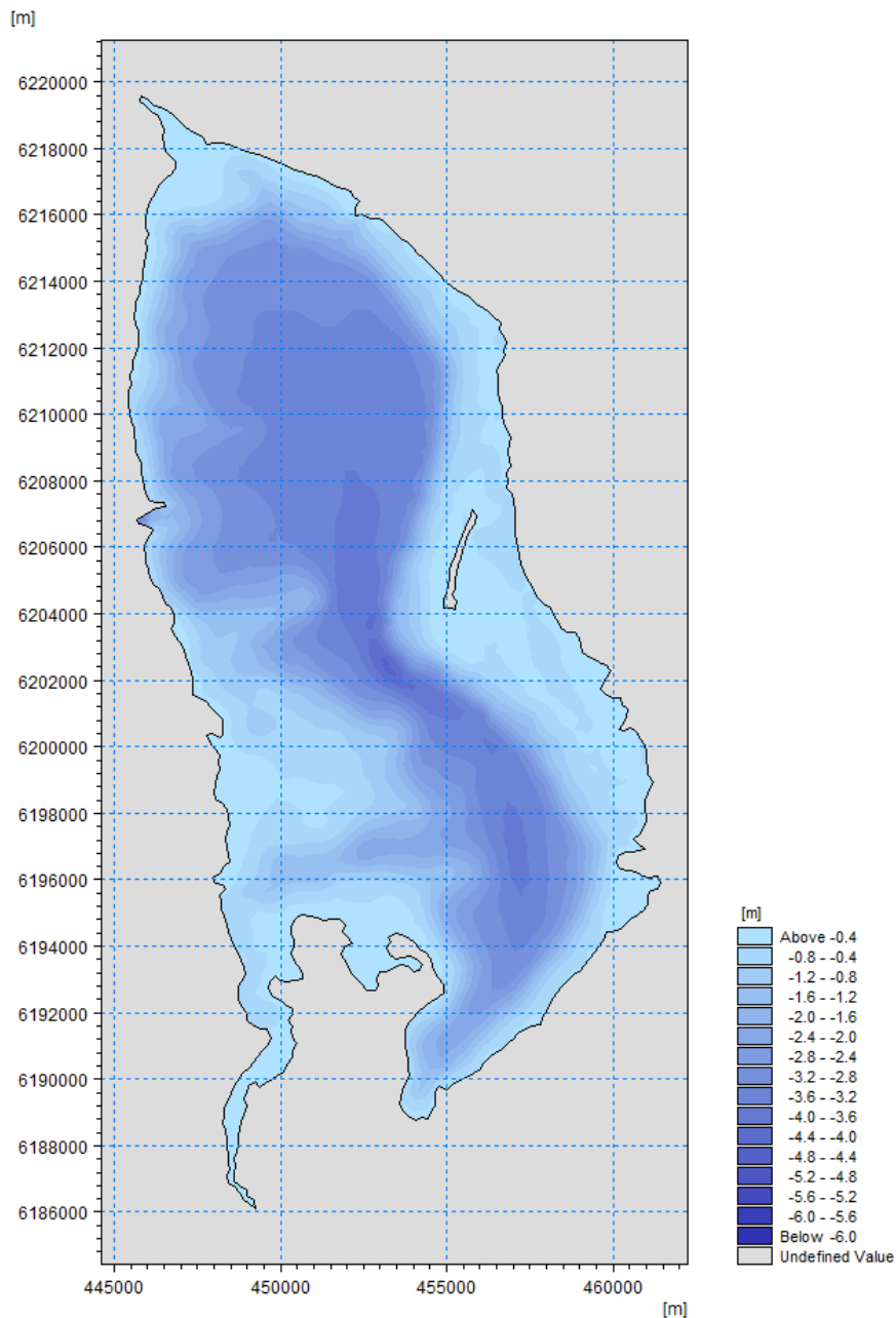
Figure 4-1 Model bathymetry of the Ringkøbing Fjord model. Water depths refer to MSL. The model has no open boundary. The sluice at Hvide Sande is implemented as a source/sink.
