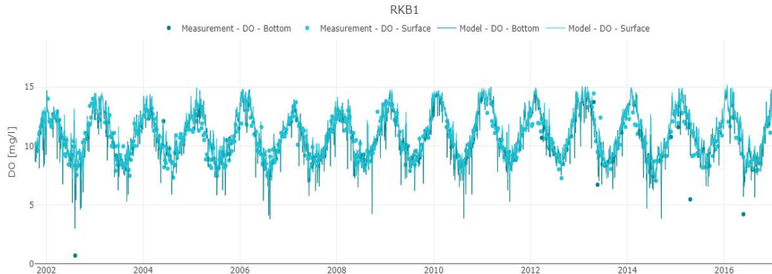
Figure 5-6 Comparison of measured and modelled concentrations of dissolved oxygen (DO, mg/l) at station RKB1 in the surface and bottom (3 m) waters. Dots represent measurements, and the solid line shows modelled data for the entire period.
