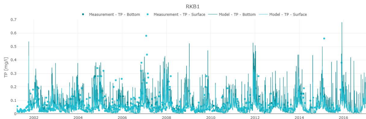
Figure 5-12 Comparison of measured and modelled concentrations of total P (TP, mg/l) at station RKB1 in surface and bottom (3 m) waters. Scatter data represent measurements, and solid lines show modelled data for the entire period.
