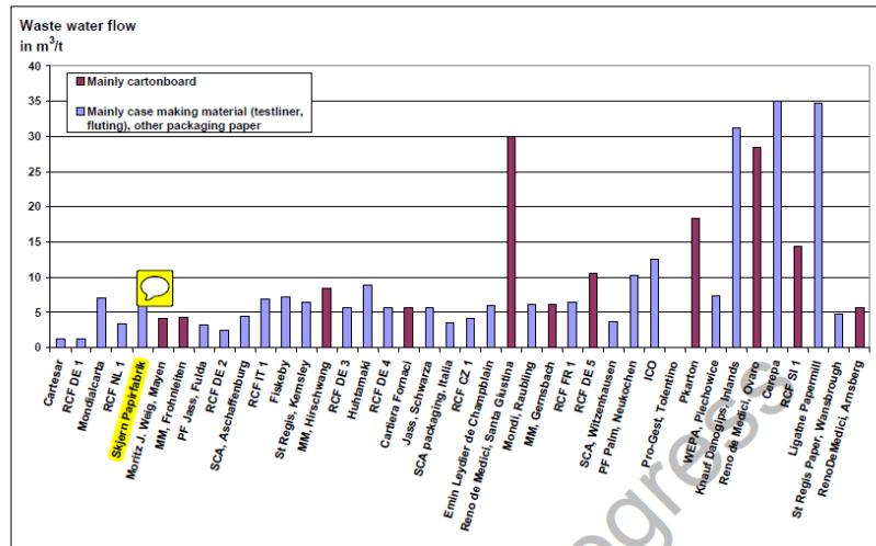
Figure 6.10: Specific waste water flow of European RCF paper mills without deinking SIDE 7
